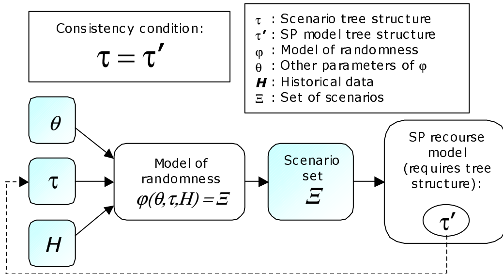
Figure 7. Scenario Generation Parameter Pairing and Tree Consistency
