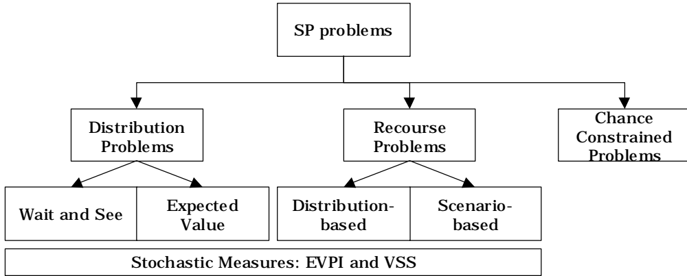
Figure 2 Taxonomy of SP problems.
