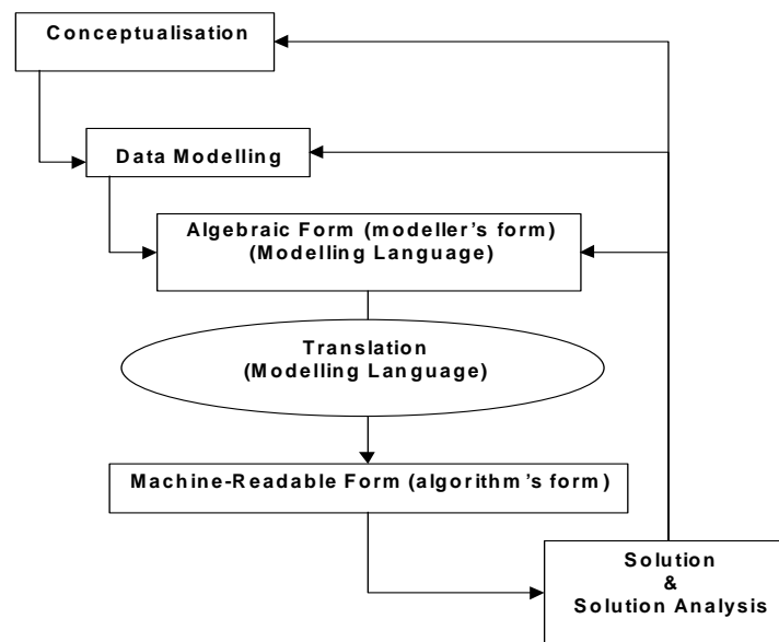
Figure 1. The modelling process.
