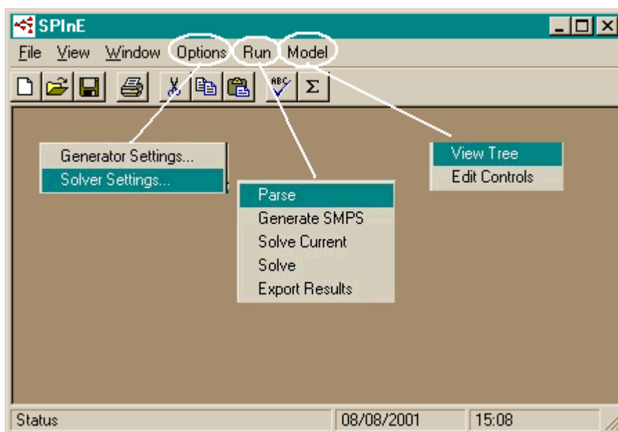
Figure 16. SPInE's menu commands
