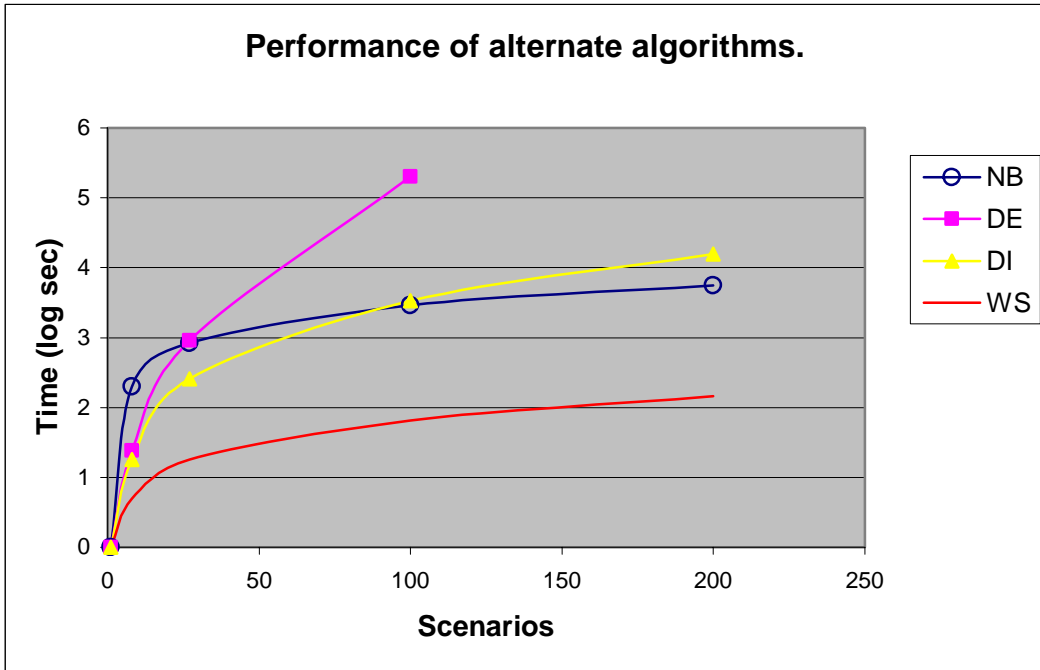
Figure 10. Performance of the algorithms on the STORM model.
