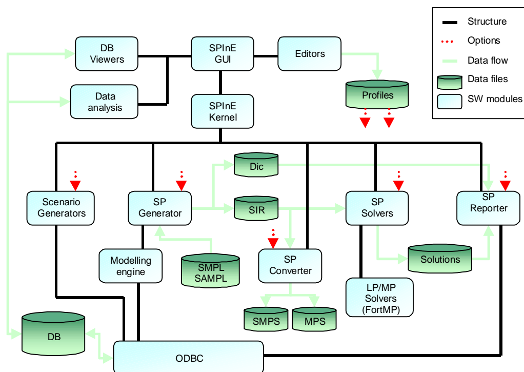
Figure 14. Software architecture of SPInE.
