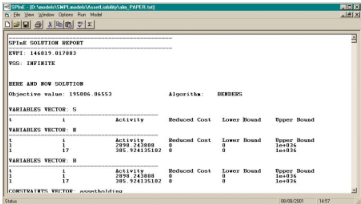
Figure 21. Text report of the optimal values
