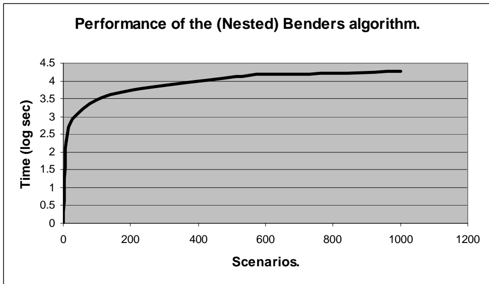
Figure 11. Performance of the (Nested) Benders on the STORM model.
