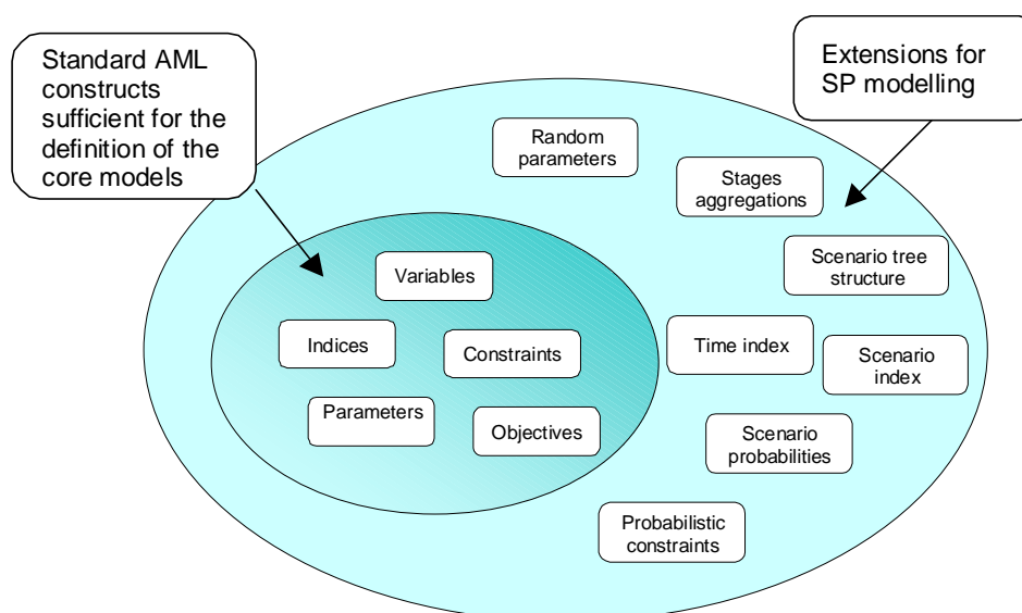
Figure 6. Extended language constructs
