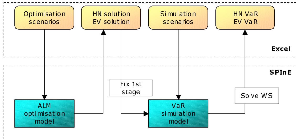
Figure 22. Computation of VaR using SPIInE and spreadsheets
