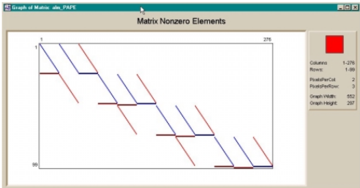
Figure 19. Matrix structure of the core LP problem
