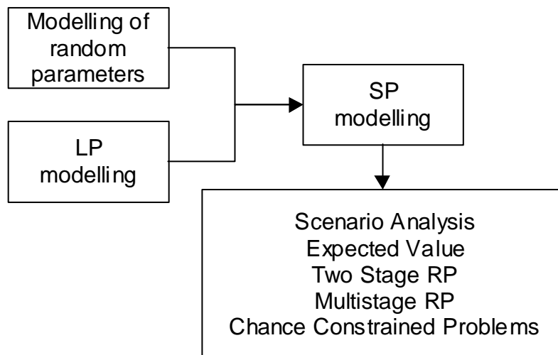
Figure 5. The combined paradigm
