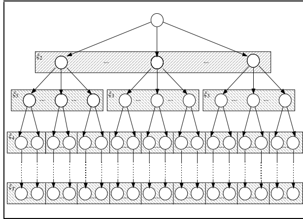
Figure 3. Event tree and scenarios
