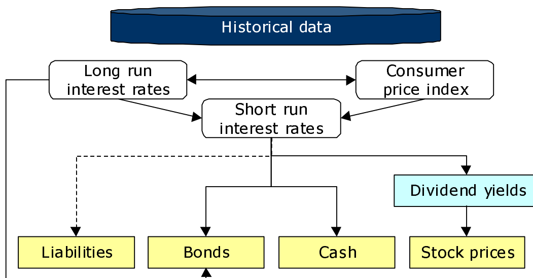
Figure 8. Asset prices generator: architecture
