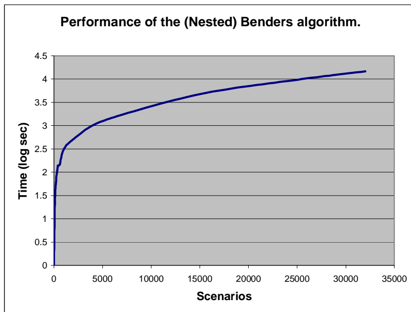
Figure 13. Performance of the (Nested) Benders on the PHONE model.
