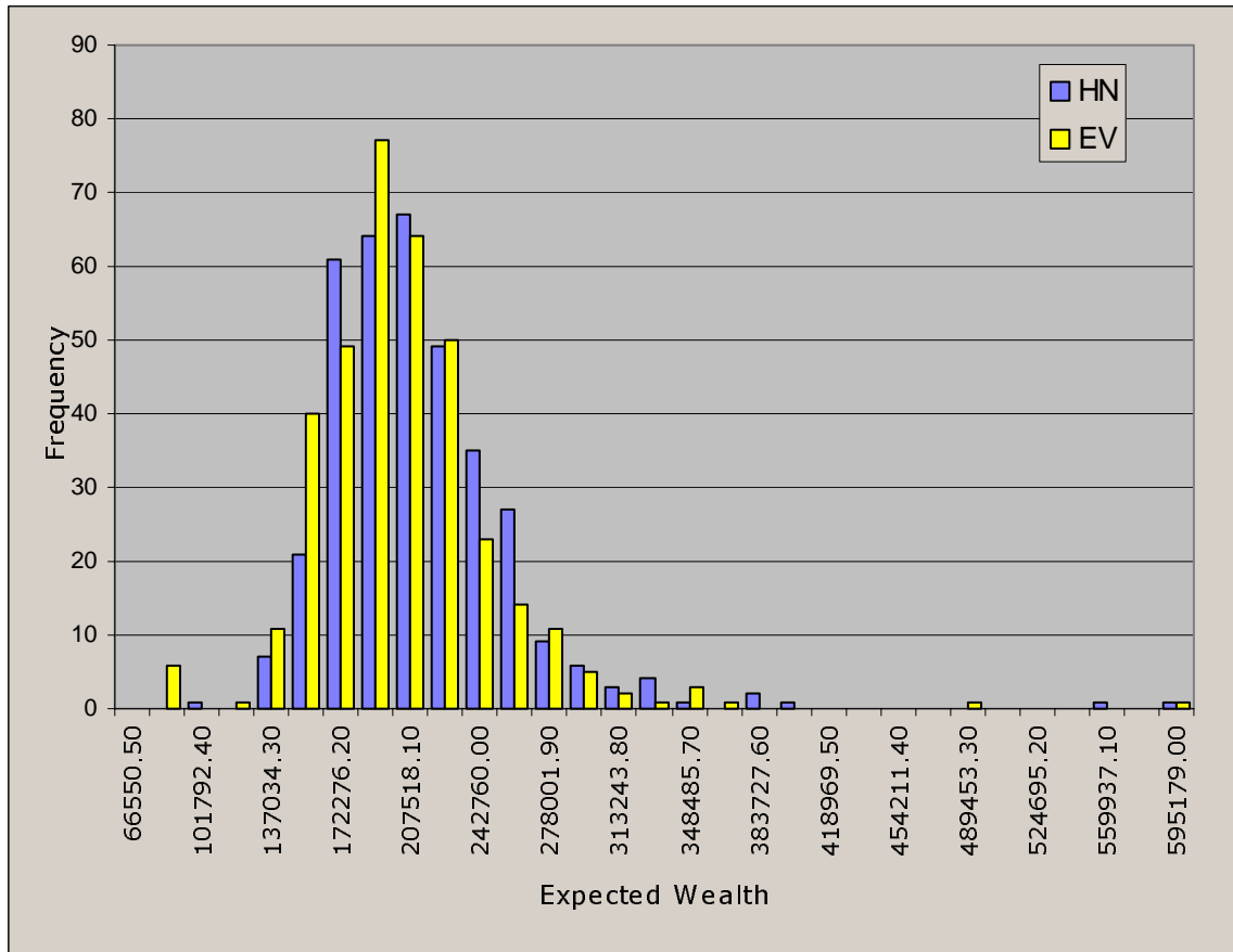
Figure 23. Distribution of the objectives for EV and HN
