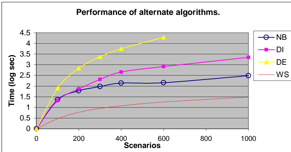
Figure 12. Performance of alternate algorithms on the PHONE model.
